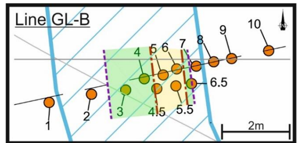
Figure 5. Section line GL-B showing broadly defined extent of infilled fissure prior to investigation (cross-hatch), conjectured extent of fissure (yellow), spalled zones (green) and probehole locations (Wardell Armstrong, 2018)
