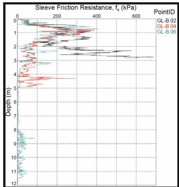
Figure 7. Examples of sleeve friction resistance responses within probeholes along section line GL-B, outside the fissure (02, black), within the spalled zone (04, red) and within the fissure (06, grey).
