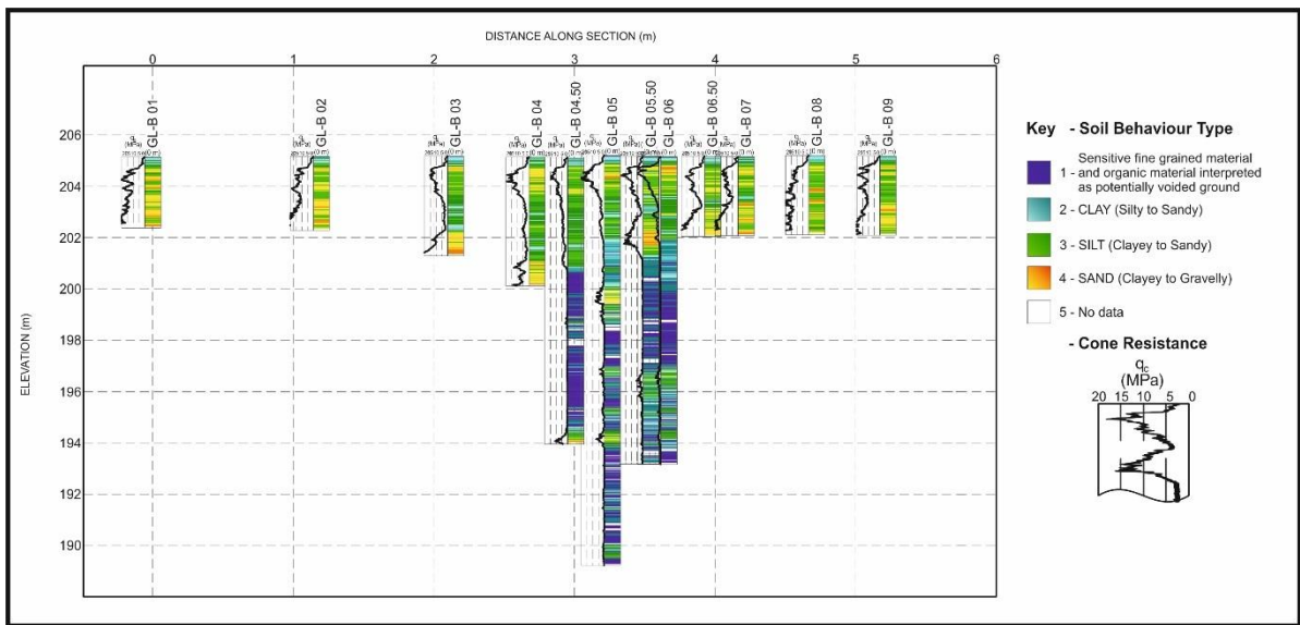
Figure 6. Cross section of line GL-B showing depth of probeholes, cone resistance values within and outside of the fissure and soil behaviour types. Produced by In Situ Site Investigation (In Situ Site Investigation, 2018) and edited by the authors
