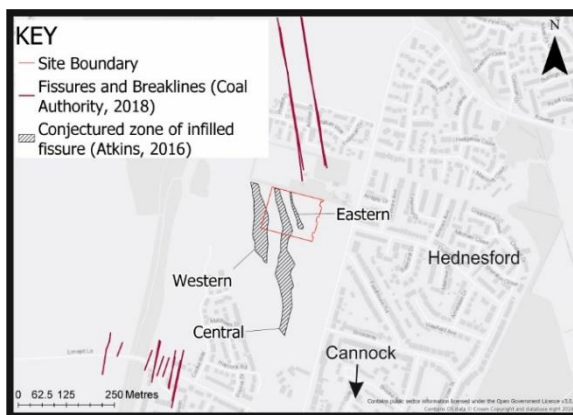
Figure 1. Site location plan showing fissures identified by previous investigations (Atkins, 2016) and The Coal Authority (Coal Authority, 2018)
