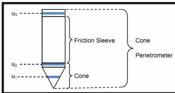
Figure 3. A simplified schematic of the cone tip and the pore pressure filter locations (In Situ Site Investigation, 2018)
